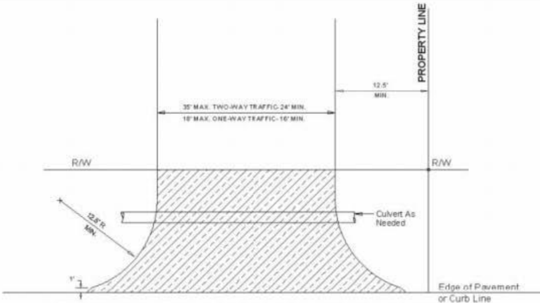
RESIDENTIAL DRIVE-LOCAL STREET N.T.S.
