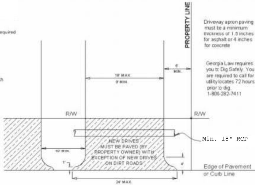
RESIDENTIAL DRIVE-LOCAL STREET N.T.S.
